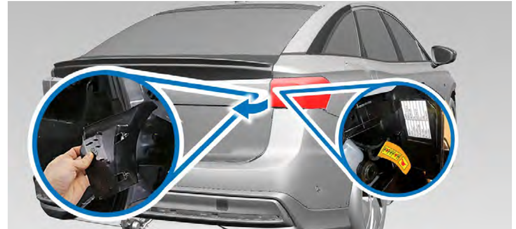
Variant 2: alternatively, the trim under the tail light can be unplipped and the cut-out connection cut.
