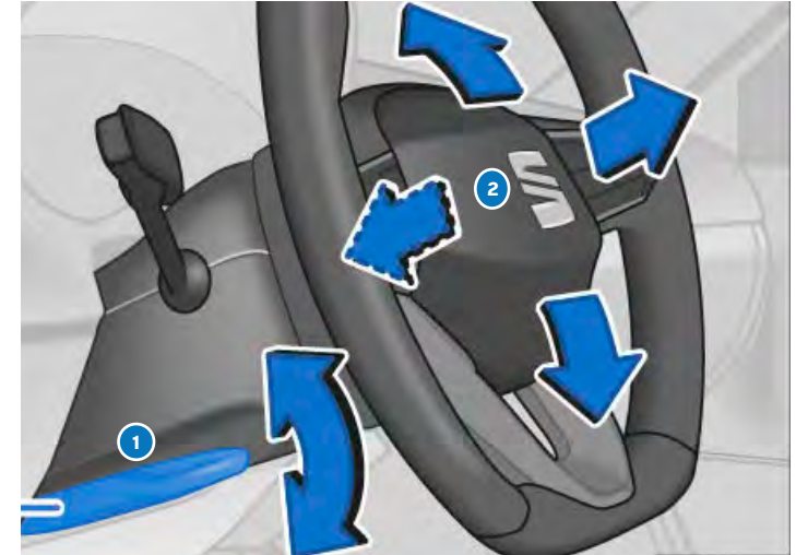
Mechanical steering column adjustment
