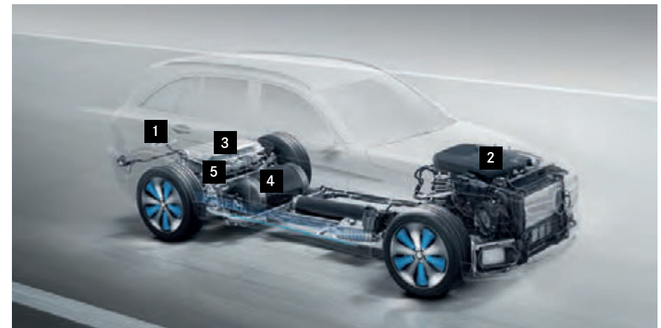
Location of fuel cell system using the GLC F-CELL as an example
