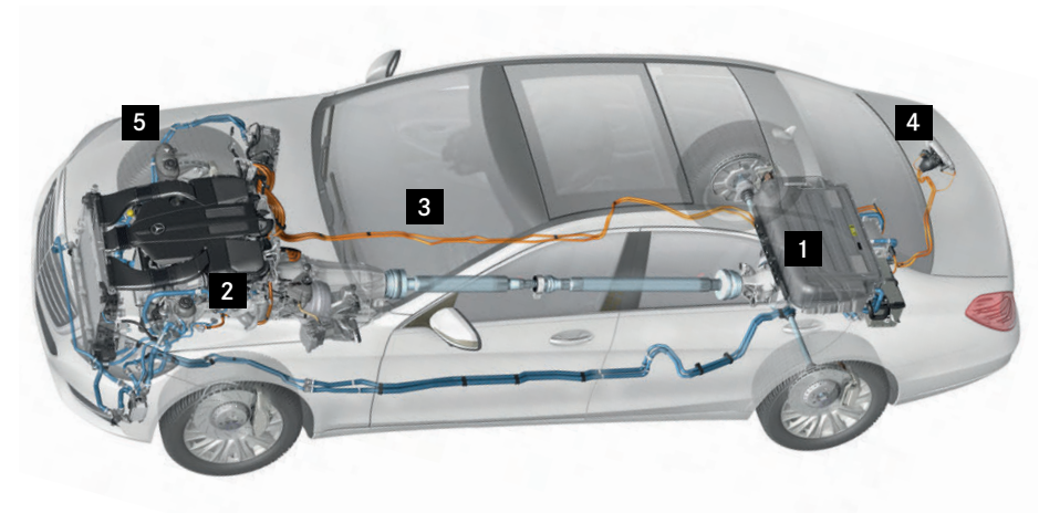
Using an S500 plug-in hybrid as an example
