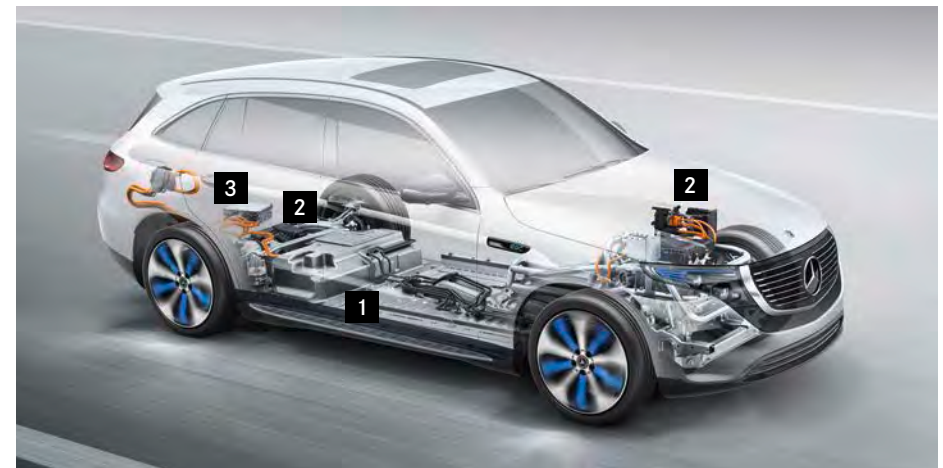
Installation positions of components using Mercedes-Benz EQC as an example.
