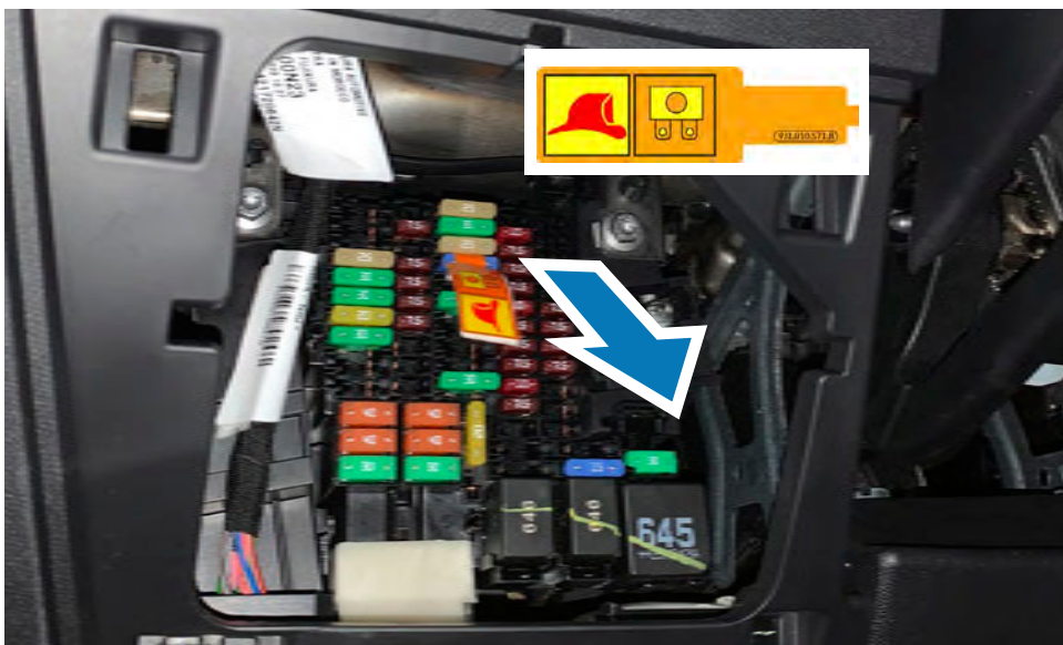
Cut-out connection in the passenger compartment, fuse carrier in the dash panel. See also old identification (previous to León 2024) .
