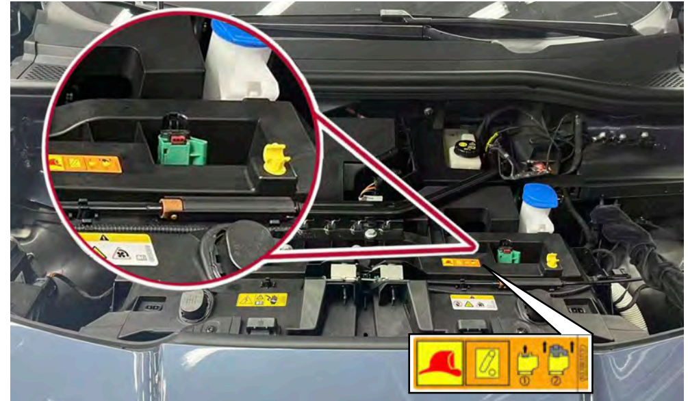
Cut-out connection in front end of electric vehicles. For vehicles before Tavascan, see also previous identification .
