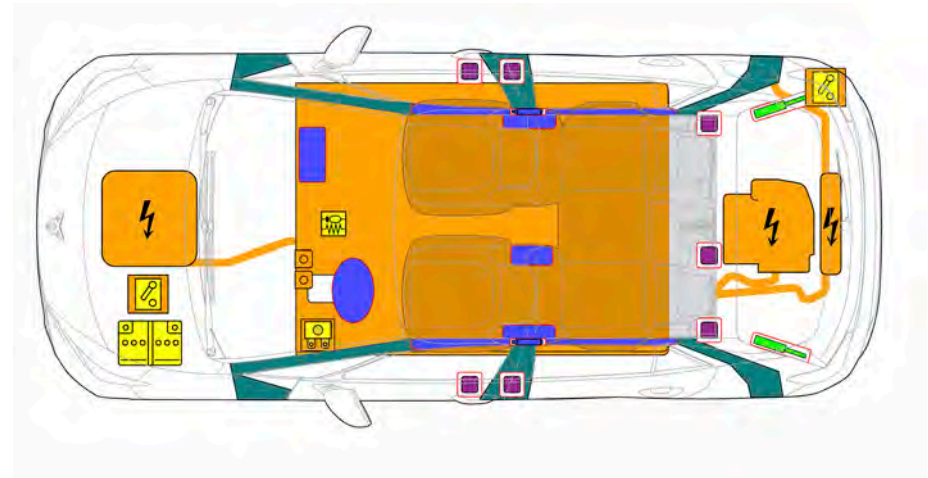
Fitting location of the high-voltage battery in the BORN
