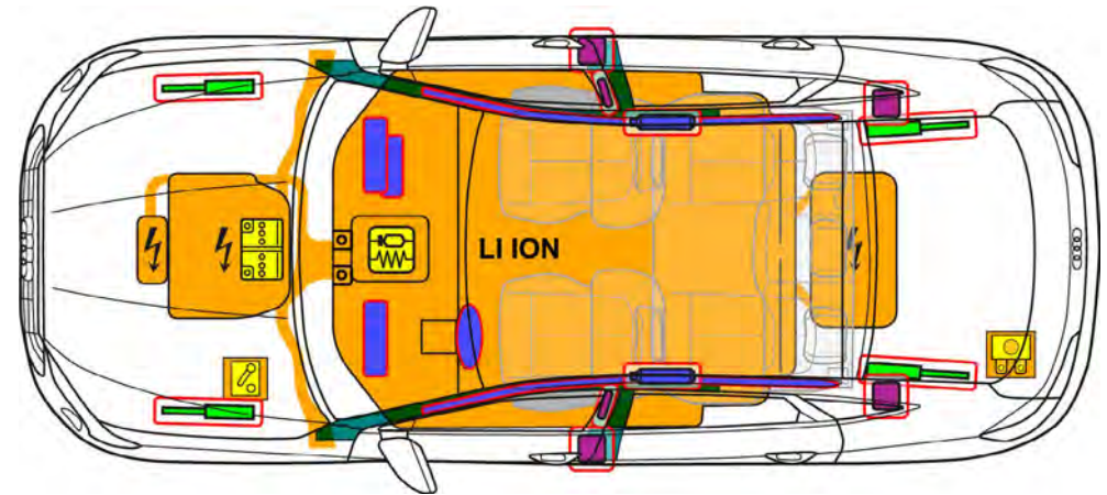
Rescue card for the Audi e-tron
