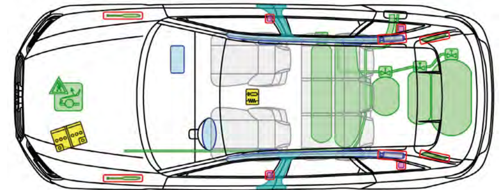
Rescue card for Audi A4 g-tron (does not comply with the current version of ISO 17840)
