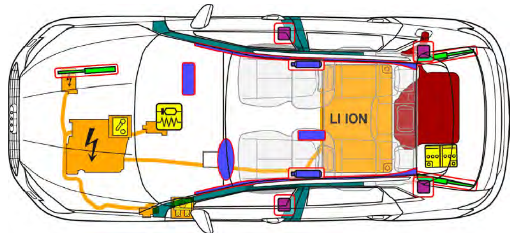
Rescue card for the Audi A3 TFSI e
