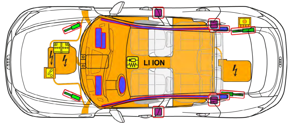
Rescue card for the e-tron GT
