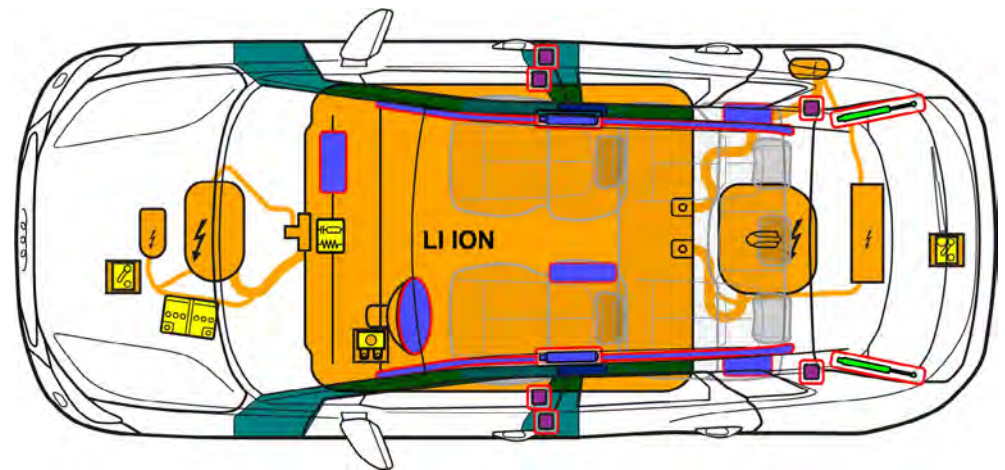
Rescue card for the Audi Q4 e-tron
