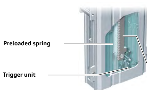
Latching mechanism
