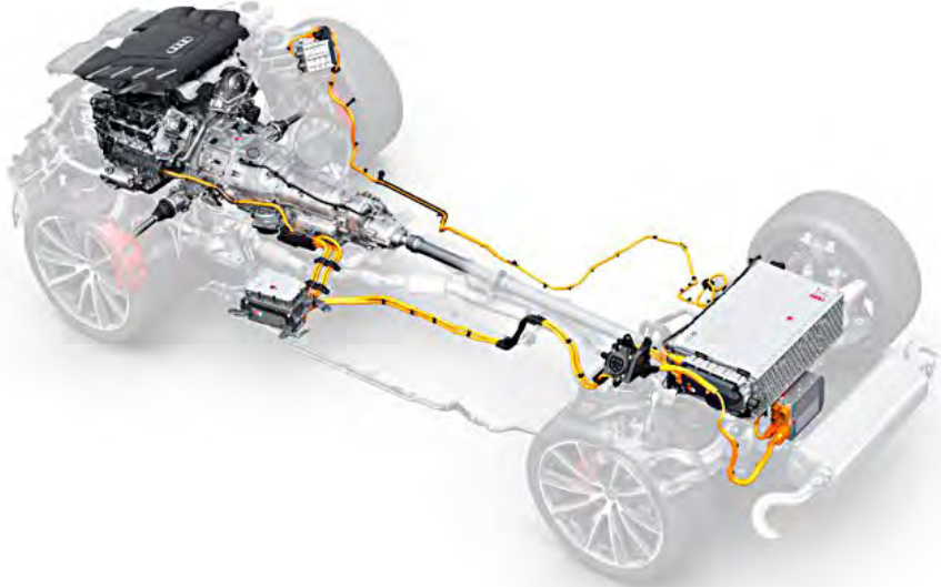
High-voltage battery in the rear of the vehicle (Audi Q8 TFSI e)
